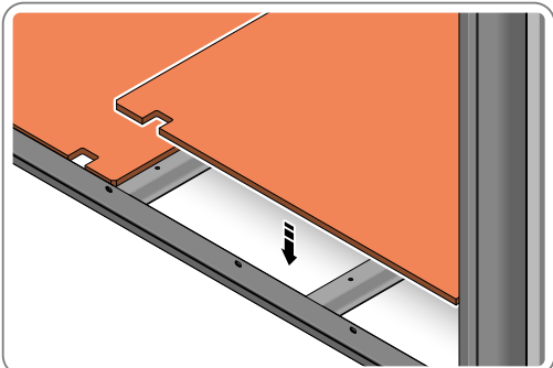
LOCATE EACH FLOOR PANEL 0203-42 INTO BASE OF STORAGE UNIT AS SHOWN.
