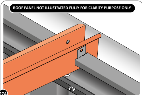
27A LOCATE ROOF ASSEMBLY ONTO ROOF FRAME, ENSURE EACH ROOF BRACE IS LOCATED INTO FRONT AND REAR ROOF INFILL AIR BEND TABS AS SHOWN.
