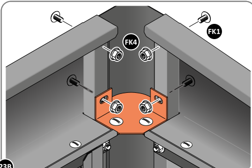
23B SECURE EACH CORNER BRACKET AND ROOF INFILL AS SHOWN ABOVE.
