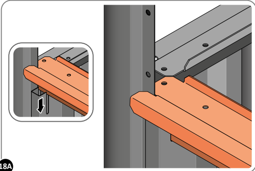
18A LOCATE LONG TOP RAIL 0203-16 AS SHOWN ABOVE.
