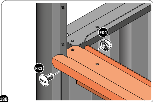
18B LOOSELY ATTACH AT x2 LOCATIONS INDICATED.
