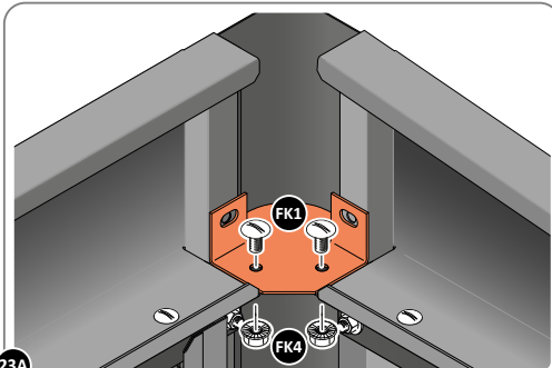
23A LOCATE AND SECURE TOP RAIL CORNER BRACKETS 0203-15 IN EACH CORNER OF THE SHED USING THE TYPICAL FIXING METHOD SHOWN ABOVE.
