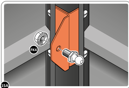
15A SECURE BALL STUD 0205-68 ONTO BOTTOM GAS STRUT BRACKET AS SHOWN.
