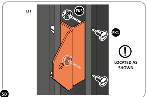
5B SECURE BOTTOM GAS STRUT BRACKET 0206-39 AS SHOWN.
