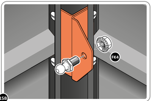
15B SECURE BALL STUD 0205-68 ONTO BOTTOM GAS STRUT BRACKET AS SHOWN.
