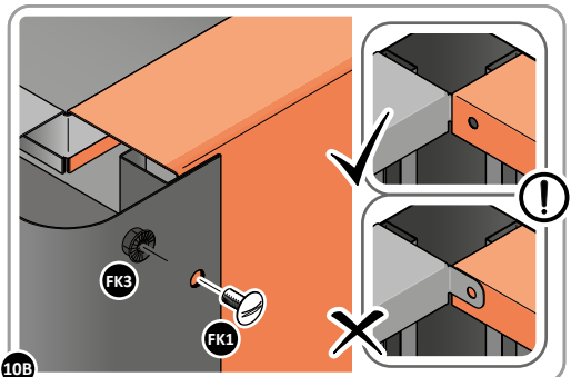
10B LOOSELY ATTACH SIDE PANEL AT EACH LOCATION INDICATED AS SHOWN.
