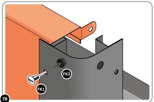
7B LOOSELY ATTACH FRONT PANEL AT EACH LOCATION INDICATED AS SHOWN.
