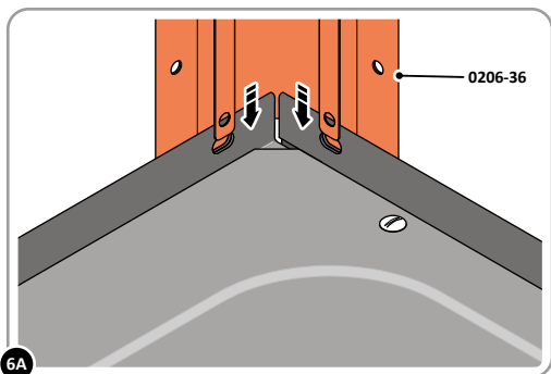
6A SLIDE EACH CORNER POST 0206-36 INTO POSITION AS SHOWN ABOVE.
