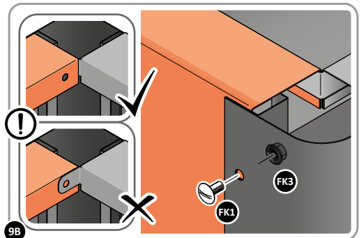
9B LOOSELY ATTACH SIDE PANEL AT EACH LOCATION INDICATED AS SHOWN.
