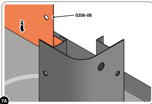
7A SLIDE FRONT PANEL 0206-08 INTO POSITION AS SHOWN ABOVE.
