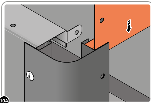
10A SLIDE SIDE PANEL 0206-09 INTO POSITION AS SHOWN ABOVE.
