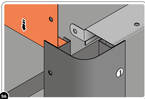
9A SLIDE SIDE PANEL 0206-09 INTO POSITION AS SHOWN ABOVE.
