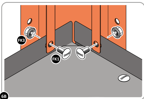
6B LOOSELY ATTACH EACH CORNER POST AS SHOWN ABOVE.
