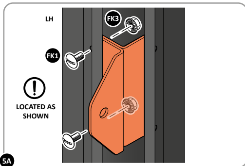
5A SECURE BOTTOM GAS STRUT BRACKET 0206-39 AS SHOWN.
