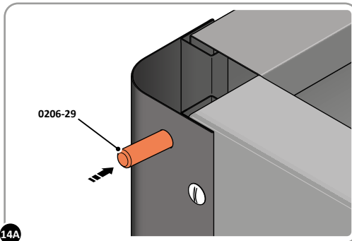
LOCATE RODS 0206-29 INTO CORNER POST APERTURES AS SHOWN.
