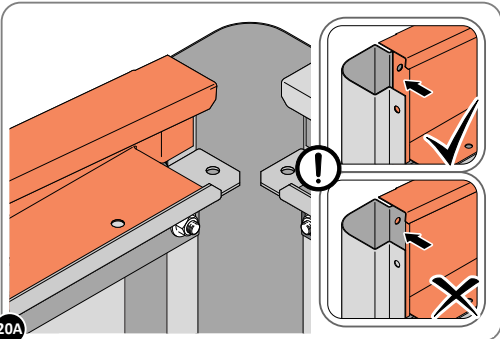
LOCATE ROOF LEFT-HAND SIDE INFILL 0203-24 AS SHOWN ABOVE.
