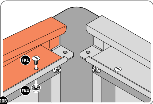
SECURE ROOF SIDE INFILL AT x4 LOCATIONS INDICATED AS SHOWN ABOVE.
