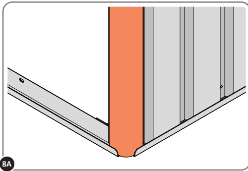
8A LOCATE CORNER POST 0205-14 (1885mm) AS SHOWN ABOVE.
