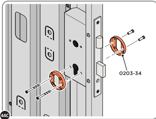
44C LOCATE AND SECURE EURO ESCUTCHEON 0203-34 AS SHOWN.
