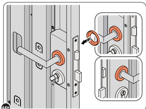
44H LOCATE COVER ONTO DOOR HANDLE AS SHOWN. PLEASE NOTE: THESE ARE PUSHED ON AND WILL CLICK INTO PLACE.
