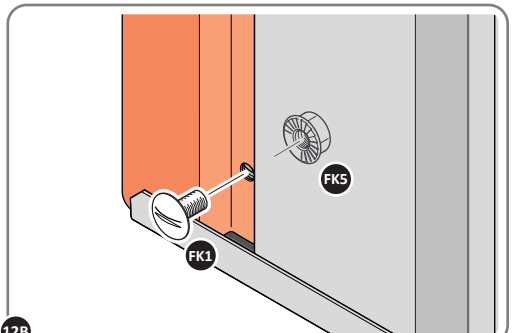
12B LOOSELY ATTACH CORNER POST AT LOCATIONS INDICATED ONLY. IMPORTANT: DO NOT SECURE AT UPPER FIXING POINT AT THIS STAGE.
