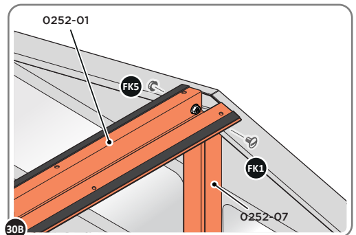
30B SECURE ROOF CHANNEL ASSEMBLY TO LONG ROOF SUPPORT 0252-07 FIXING POINT (x2 EACH SIDE) USING FASTENERS DETAILED ABOVE.
