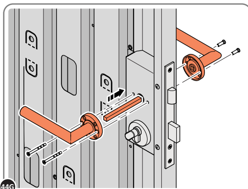
44G LOCATE AND SECURE DOOR HANDLE ASSEMBLY 0203-33 AS SHOWN.
