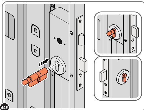
44E LOCATE EURO CYLINDER 0203-36 INTO DOOR APERTURE. IMPORTANT: ENSURE COVER IS FITTED AS SHOWN.
