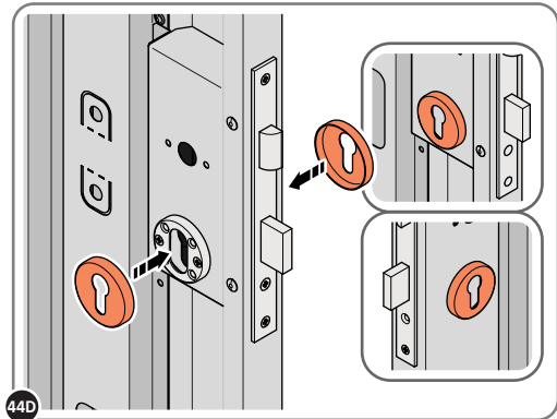
44D LOCATE EURO ESCUTCHEON COVER 0203-34 ONTO EURO ESCUTCHEON AS SHOWN. PLEASE NOTE: THESE ARE PUSHED ON AND WILL CLICK INTO PLACE.
