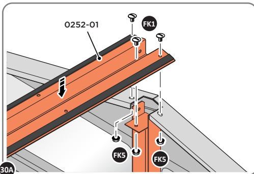
30A SLOT ROOF CHANNEL ASSEMBLY 0252-01 INTO ROOF SUPPORT. FIXING POINT (x3 EACH SIDE) USING FASTENERS DETAILED ABOVE.
