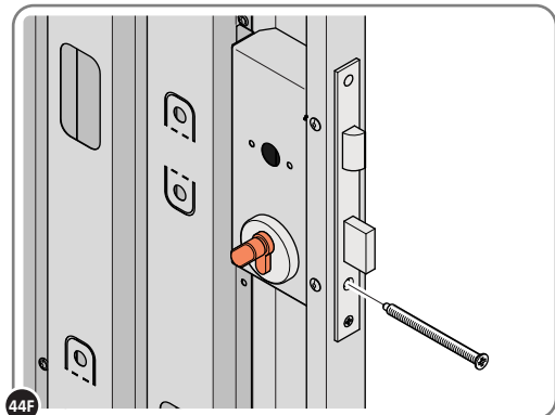
44F SECURE EURO CYLINDER 0203-36 AS SHOWN ABOVE. PLEASE NOTE: FIXING IS PART OF THE EURO MORTICE LOCK ASSEMBLY.
