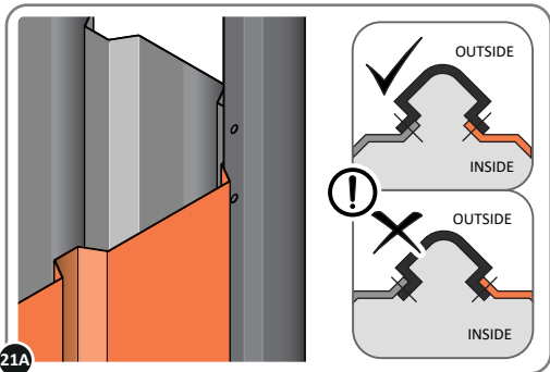
21A LOCATE WALL PANEL 0213-03 (1850 x 324mm) AS SHOWN ABOVE. IMPORTANT: ENSURE PANEL IS IN THE CORRECT ORIENTATION.
