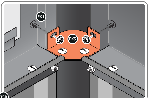
SECURE EACH CORNER BRACKET AND ROOF INFILL AS SHOWN ABOVE.
