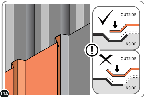
11A LOCATE WALL PANEL 0205-12 INTO POSITION AS SHOWN ABOVE. IMPORTANT: ENSURE PANEL IS IN THE CORRECT ORIENTATION.
