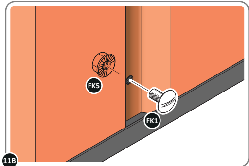
11B LOOSELY ATTACH BACK WALL PANEL AT x3 LOCATIONS INDICATED ONLY. IMPORTANT: DO NOT SECURE ANY FIXING POINTS OTHER THAN THOSE INDICATED.
