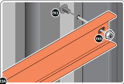
LOCATE AND LOOSELY ATTACH SHORT CENTRE BRACE 0213-04 AS SHOWN AT LOCATION INDICATED ABOVE.
