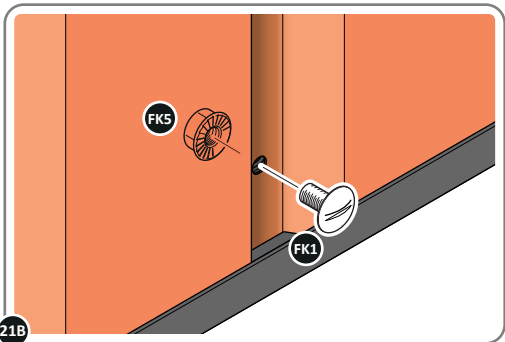
21B LOOSELY ATTACH WALL PANEL AT x 2 LOCATIONS INDICATED ONLY. IMPORTANT: DO NOT SECURE ANY FIXING POINTS OTHER THAN THOSE INDICATED.
