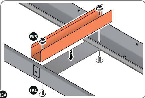
LOCATE AND SECURE WINDOW SUPPORTS 0205-44 TO WINDOW ASSEMBLY 0213-14 AS SHOWN ABOVE.
