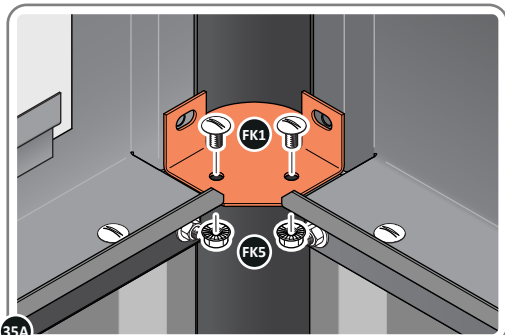
LOCATE AND SECURE TOP RAIL CORNER BRACKETS 0203-15 IN EACH CORNER OF THE SHED USING THE TYPICAL FIXING METHOD SHOWN ABOVE.
