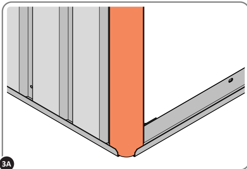
3A LOCATE CORNER POST 0205-14 AS SHOWN ABOVE.
