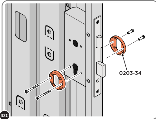
42C LOCATE AND SECURE EURO ESCUTCHEON 0203-34 AS SHOWN.
