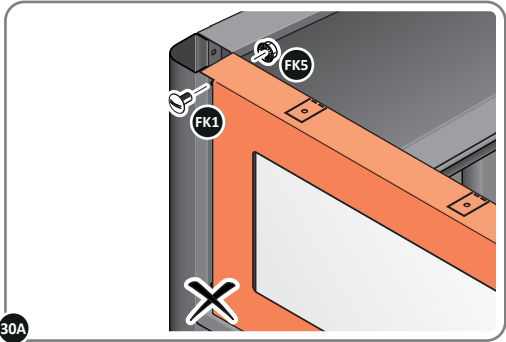
SECURE ROOF FRONT INFILLS AT x2 LOCATIONS INDICATED.
