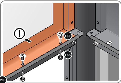
SECURE WINDOW ASSEMBLY AT x10 LOCATIONS INDICATED AS SHOWN ABOVE.
