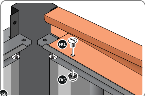
26B SECURE ROOF SIDE INFILL AT LOCATIONS INDICATED AS SHOWN ABOVE.
