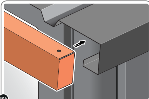
LOCATE ROOF CAP 0215-03 ONTO FRONT OF ROOF.
