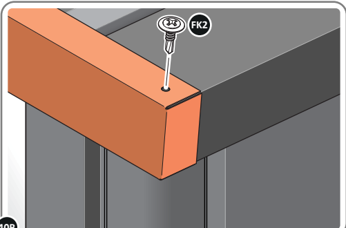
SECURE ROOF CAP AT x10 LOCATIONS INDICATED USING TYPICAL FIXING METHOD. PLEASE NOTE: THE FIXING USED IS A SELF DRILLING COMPONENT.
