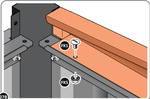
SECURE ROOF SIDE INFILL AT LOCATIONS INDICATED AS SHOWN ABOVE.
