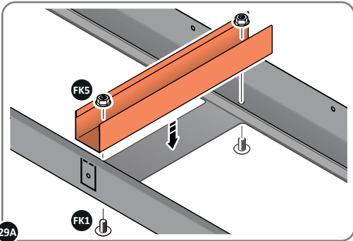
LOCATE AND SECURE WINDOW SUPPORT 0205-44 TO WINDOW ASSEMBLY 0215-12 AS SHOWN ABOVE.
