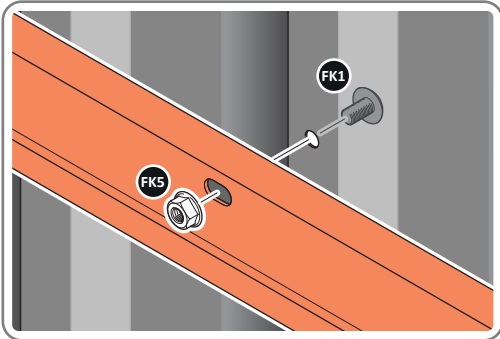
LOCATE AND LOOSELY ATTACH MID CENTRE BRACE 0212-03 AS SHOWN AT x3 LOCATIONS INDICATED ABOVE.
