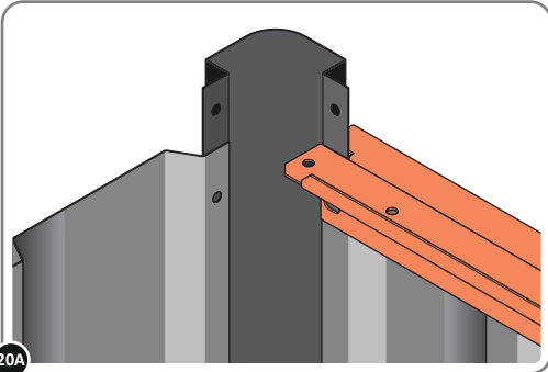
20A LOCATE SHORT ROOF RAIL 0215-02 AS SHOWN ABOVE.
