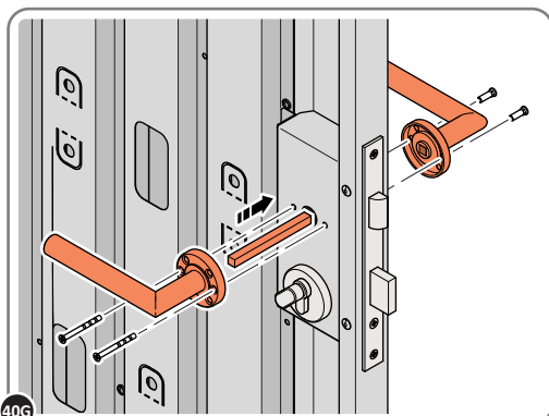
40G LOCATE AND SECURE DOOR HANDLE ASSEMBLY 0203-33 AS SHOWN.
