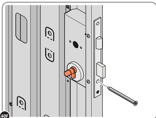
40F SECURE EURO CYLINDER 0203-36 AS SHOWN ABOVE. PLEASE NOTE: FIXING IS PART OF THE EURO MORTICE LOCK ASSEMBLY.
