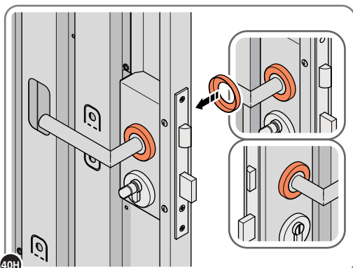
40H LOCATE COVER ONTO DOOR HANDLE AS SHOWN. PLEASE NOTE: THESE ARE PUSHED ON AND WILL CLICK INTO PLACE.
