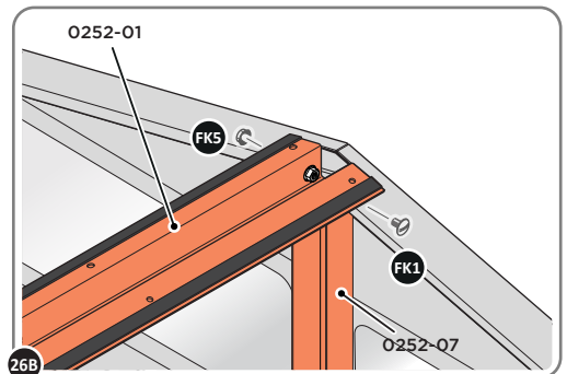
26B SECURE ROOF CHANNEL ASSEMBLY TO LONG ROOF SUPPORT 0252-07 FIXING POINT (x2 EACH SIDE) USING FASTENERS DETAILED ABOVE.
