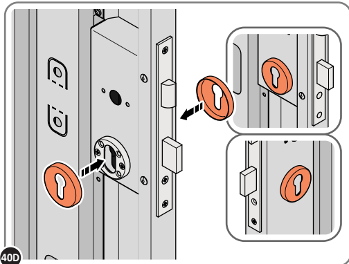
40D LOCATE EURO ESCUTCHEON COVER 0203-34 ONTO EURO ESCUTCHEON AS SHOWN. PLEASE NOTE: THESE ARE PUSHED ON AND WILL CLICK INTO PLACE.
