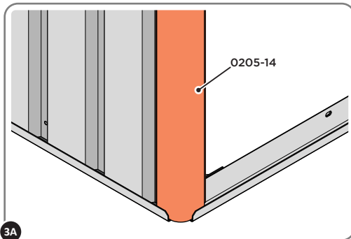
3A LOCATE CORNER POST 0205-14 (1885mm) AS SHOWN ABOVE.
