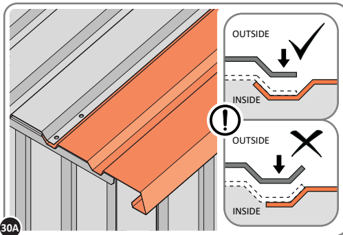
30A ALIGN AND OVERLAP ROOF PANEL 0244-06 WITH ROOF PANEL SIDE AS SHOWN.
