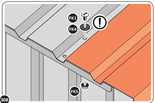
30B SECURE ROOF PANELS AT x 3 LOCATIONS INDICATED USING TYPICAL FIXING METHOD.
