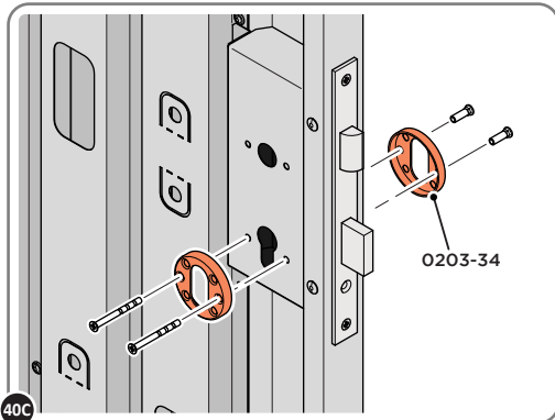
40C LOCATE AND SECURE EURO ESCUTCHEON 0203-34 AS SHOWN.
