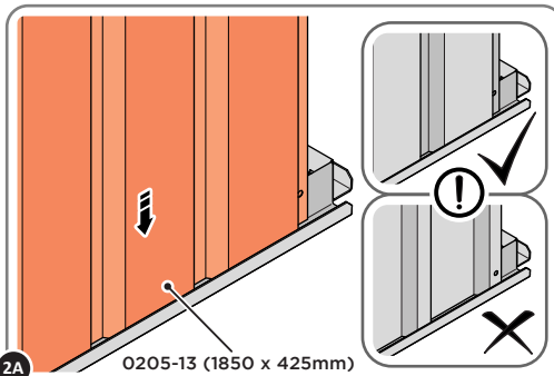
2A LOCATE WALL PANEL 0205-13 (1850 x 425mm)
