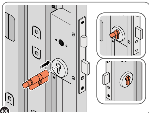
40E LOCATE EURO CYLINDER 0203-36 INTO DOOR APERTURE. IMPORTANT: ENSURE COVER IS FITTED AS SHOWN.
