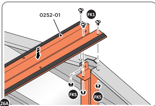
26A SLOT ROOF CHANNEL ASSEMBLY 0252-01 INTO ROOF SUPPORT. FIXING POINT (x3 EACH SIDE) USING FASTENERS DETAILED ABOVE.
