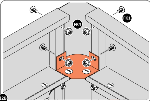
22B SECURE EACH CORNER BRACKET AND ROOF INFILL AS SHOWN ABOVE.
