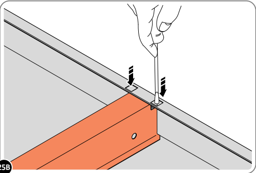
25B PUSH AIR BEND TABS DOWN TO SECURE ROOF BRACE IN POSITION.
