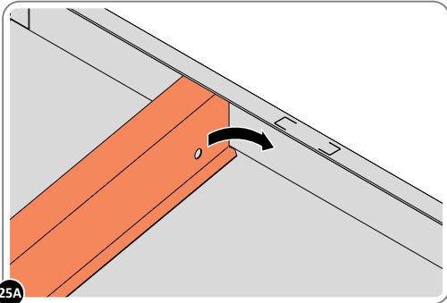
25A LOCATE EACH ROOF BRACE 0203-18 INTO ROOF 0203-20, ROTATE AND ALIGN WITH AIR BEND TABS.
