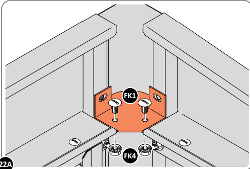
22A LOCATE AND SECURE TOP RAIL CORNER BRACKETS 0203-15 IN EACH CORNER OF THE SHED USING THE TYPICAL FIXING METHOD SHOWN ABOVE.
