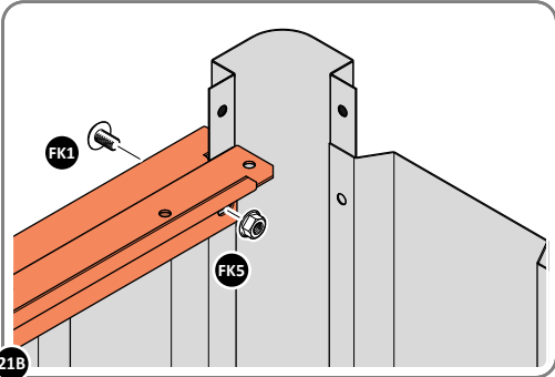
21B LOOSELY ATTACH AT x15 LOCATIONS INDICATED.
