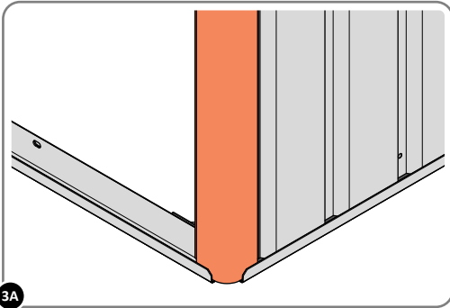
LOCATE CORNER POST 0205-14 AS SHOWN ABOVE.
