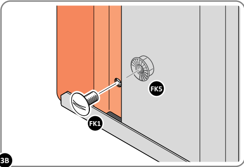
LOOSELY ATTACH CORNER POST AT LOCATION INDICATED ONLY. IMPORTANT: DO NOT SECURE AT UPPER FIXING POINT AT THIS STAGE.
