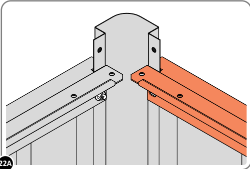
22A LOCATE LONG ROOF RAIL 0213-02 AS SHOWN ABOVE.
