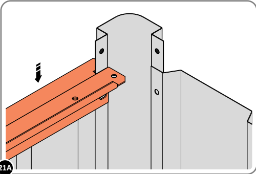
21A LOCATE SHORT ROOF RAIL 0205-18 AS SHOWN ABOVE.
