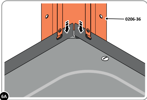
SLIDE EACH CORNER POST 0206-36 INTO POSITION AS SHOWN ABOVE.
