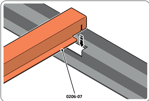
SLOT FLOOR BRACE 0206-07 INTO POSITION AS SHOWN ABOVE.
