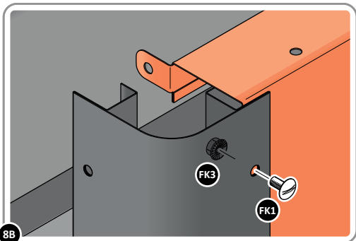
LOOSELY ATTACH REAR PANEL AT EACH LOCATION INDICATED AS SHOWN.
