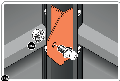
SECURE BALL STUD 0205-68 ONTO BOTTOM GAS STRUT BRACKET AS SHOWN.
