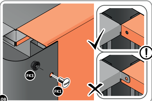
LOOSELY ATTACH SIDE PANEL AT EACH LOCATION INDICATED AS SHOWN.
