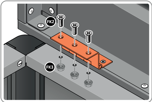
SECURE LID ASSEMBLY HINGE ONTO REAR PANEL AT EACH LOCATION INDICATED.
