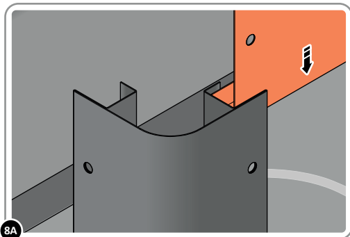
SLIDE REAR PANEL 0206-10 INTO POSITION AS SHOWN ABOVE.
