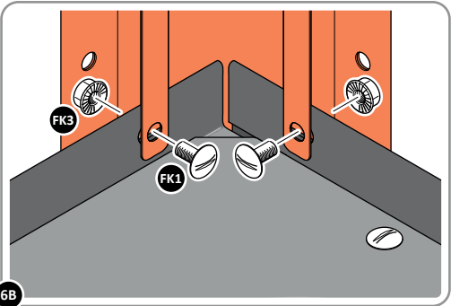
LOOSELY ATTACH EACH CORNER POST AS SHOWN ABOVE.
