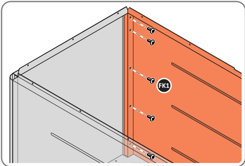
SECURE PANELS, AT LOCATIONS INDICATED ABOVE.
