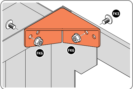
LOCATE AND SECURE CORNER FRAME BRACKET 0268-27 TO TOP FRAME. AS SHOWN ABOVE
