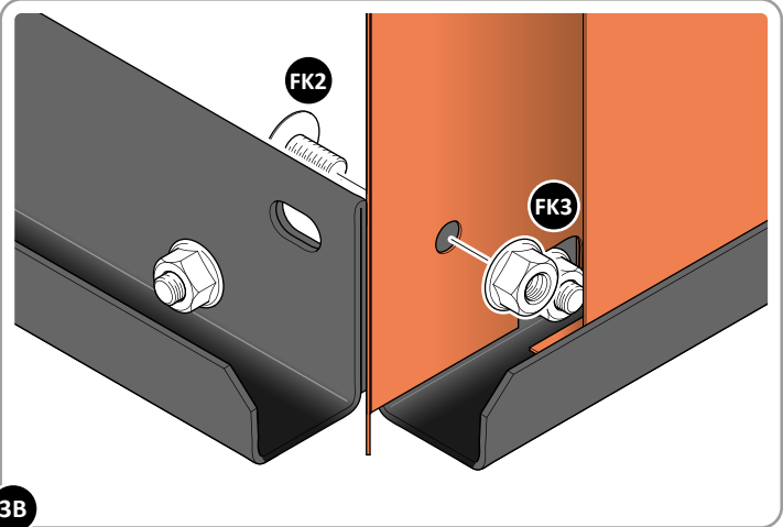
LOOSELY ATTACH BACK PANEL AT EACH LOCATION INDICATED AS SHOWN.
