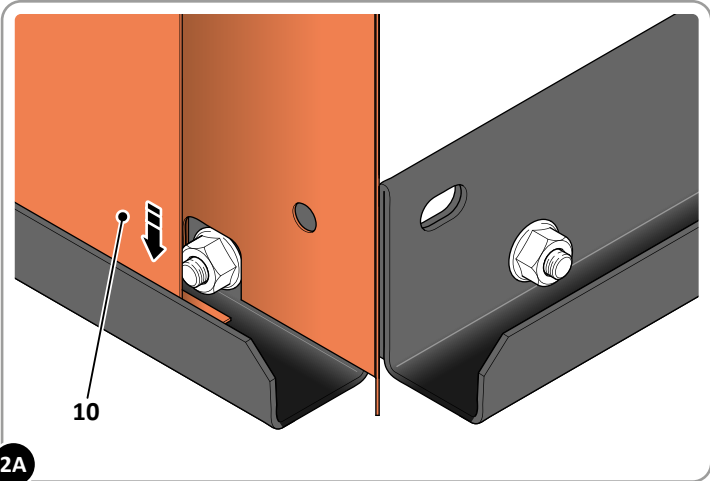
2A LOCATE FRONT PANEL (10) INTO FLOOR RAIL CHANNEL AS SHOWN ABOVE.
