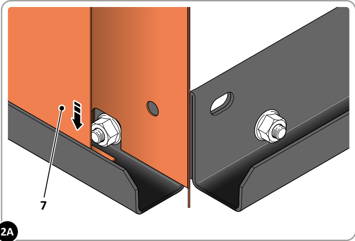
LOCATE FRONT PANEL (7) INTO FLOOR RAIL CHANNEL AS SHOWN ABOVE.
