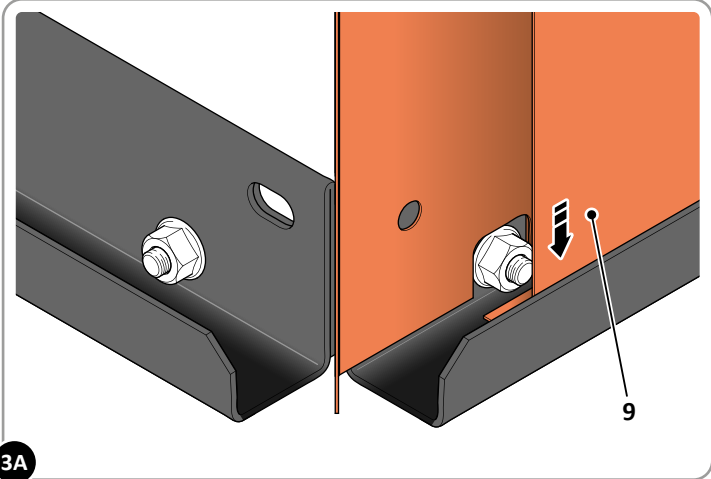
LOCATE BACK PANEL (9) INTO FLOOR RAIL CHANNEL AS SHOWN ABOVE.
