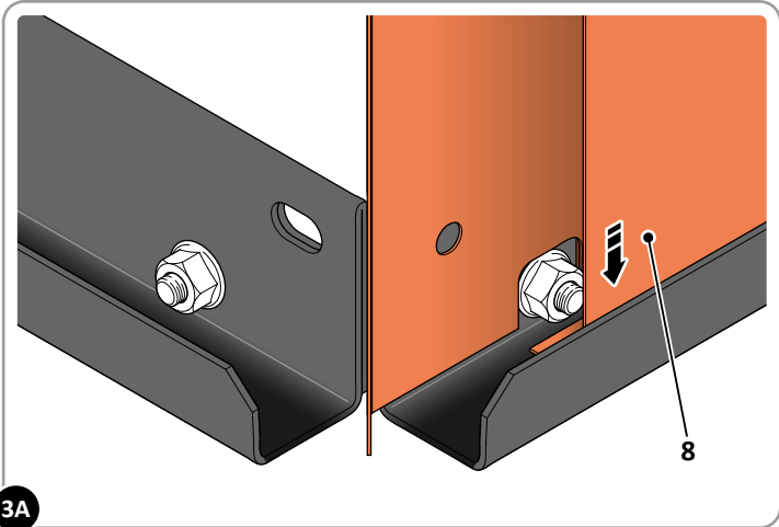
LOCATE A SIDE / BACK PANEL (8) INTO FLOOR RAIL CHANNEL AS SHOWN ABOVE.
