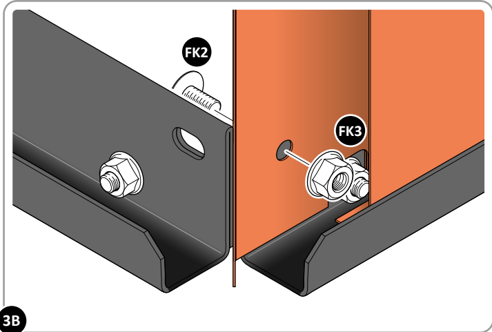
LOOSELY ATTACH PANEL AT EACH LOCATION INDICATED AS SHOWN.
