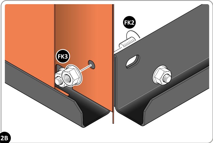
2B LOOSELY ATTACH FRONT PANEL AT EACH LOCATION INDICATED AS SHOWN.
