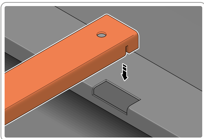
SLOT FLOOR BRACE (6) INTO FLOOR HOLDERS AS SHOWN ABOVE.
