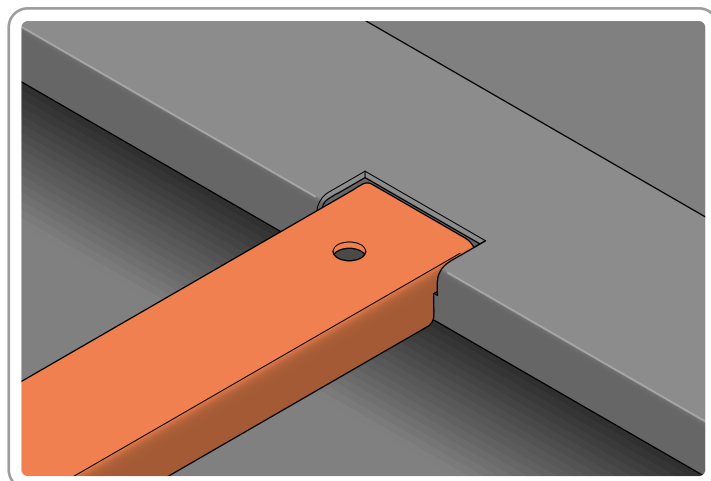
FLOOR BRACE IN POSITION
