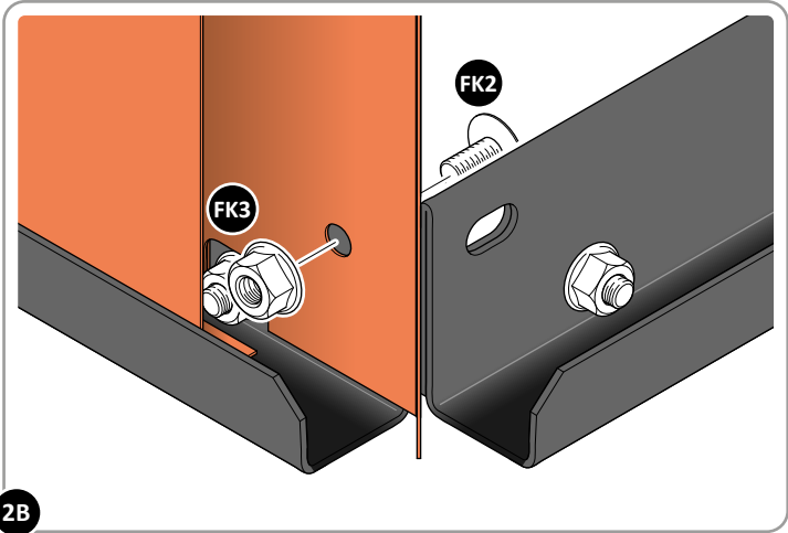
LOOSELY ATTACH FRONT PANEL AT EACH LOCATION INDICATED AS SHOWN.
