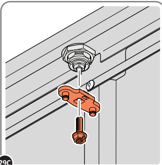
29C SECURE 2 POINT CAM 0206-28 ONTO T-HANDLE USING BOLT SHOWN ABOVE FROM T-HANDLE ASSEMBLY.
