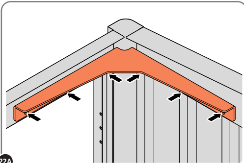
22A LOCATE AND LOOSELY ATTACH EACH TOP FRONT SUPPORT BRACKET AS SHOWN USING THE TYPICAL FIXING METHOD SHOWN.
