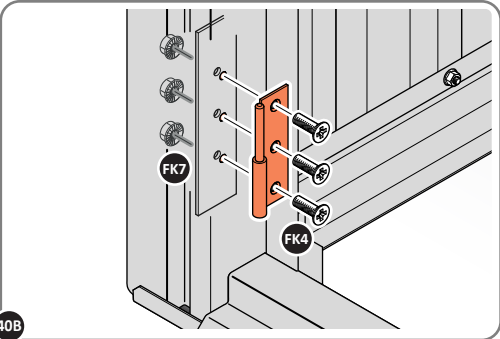
SECURE DOOR HINGE PLATE 0203-37 AND LEFT-HAND HINGE 0203-27 AS SHOWN. IMPORTANT: ENSURE CORRECT DOOR HINGE IS SECURED TO CORRECT DOOR.
