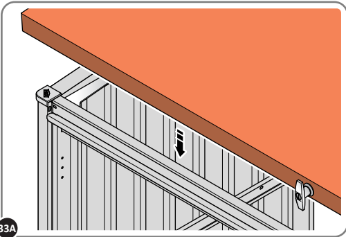
LOCATE LID ASSEMBLY ONTO STORAGE UNIT AS SHOWN.
