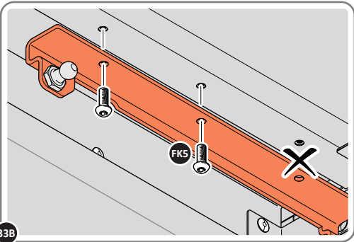
SECURE HINGE BRACKET ONTO LID ASSEMBLY, DO THIS WITH THE LID DOWN. IMPORTANT: ONLY ATTACH AT FIXING POINTS INDICATED AT THIS STAGE.
