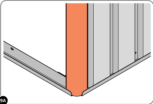
9A LOCATE CORNER POST 0205-14 AS SHOWN ABOVE.
