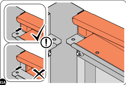
31A LOCATE ROOF SIDE INFILL 0205-31 AS SHOWN ABOVE.
