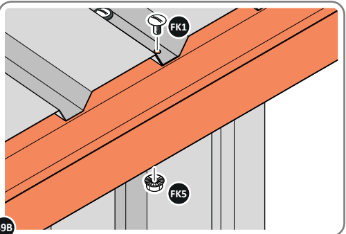
49B SECURE ROOF GUTTER AT x11 LOCATIONS INDICATED USING TYPICAL FIXING METHOD.
