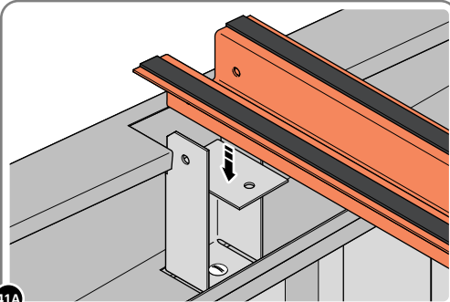
41A SLOT EACH ROOF CHANNEL ASSEMBLY 0213-06 INTO ROOF SUPPORT.
