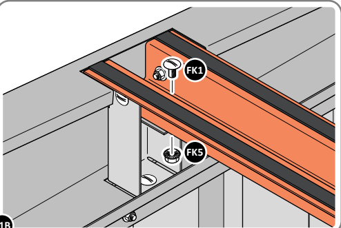
41B SECURE ROOF CHANNEL ASSEMBLY AT EACH FIXING POINT (x3 EACH SIDE) USING FASTENERS DETAILED ABOVE.
