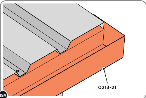
49A SLIDE ROOF GUTTER 0213-21 INTO POSITION AT THE REAR OF THE SHED ROOF.
