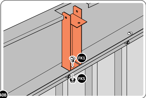
LOCATE AND SECURE LONG ROOF SUPPORT 0205-20.
