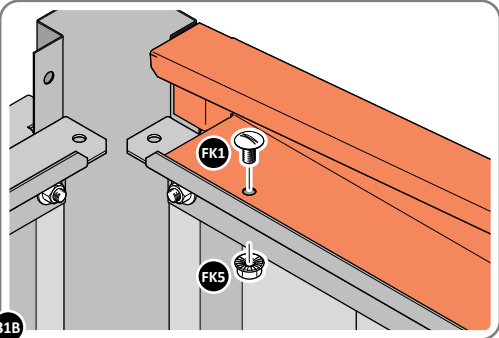
31B SECURE ROOF SIDE INFILL AT x6 LOCATIONS INDICATED, AS SHOWN ABOVE.
