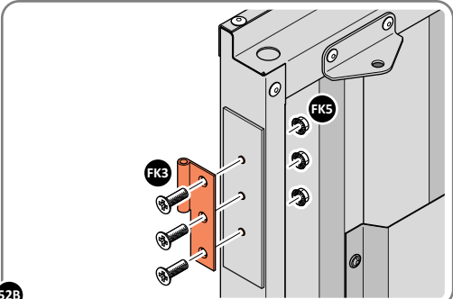
52B SECURE DOOR HINGE PLATE AND HINGE 0203-27 AND 0203-28 AS SHOWN. IMPORTANT: ENSURE CORRECT DOOR HINGE IS SECURED TO CORRECT DOOR.
