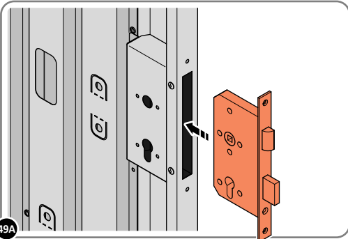
49A LOCATE EURO MORTICE LOCK 0203-32 RIGHT-HAND DOOR APERTURE AS SHOWN.
