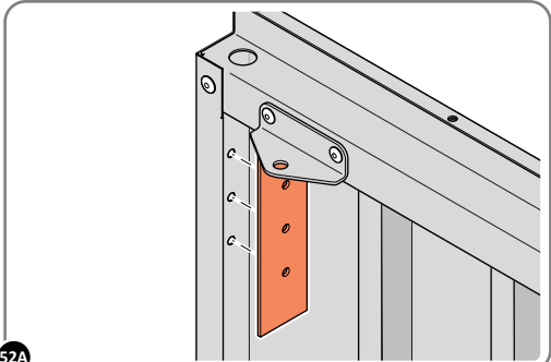
52A LOCATE DOOR HINGE PLATE 0203-37 WITHIN DOOR AS SHOWN.
