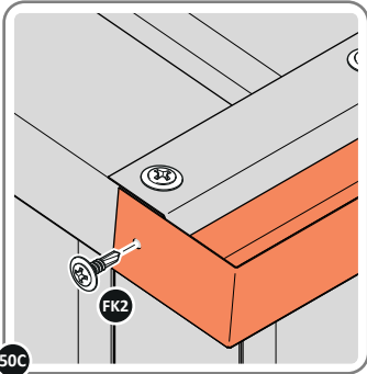
50C SECURE SLIDE ROOF GUTTER 0215-05 AT x2 LOCATIONS.
