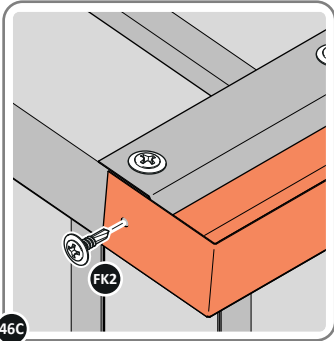
46C SECURE SLIDE ROOF GUTTER 0213-21 AT x2 LOCATIONS.
