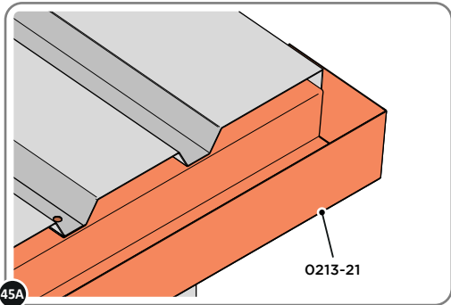
SLIDE ROOF GUTTER 0213-21 INTO POSITION AT THE REAR OF THE SHED ROOF.
