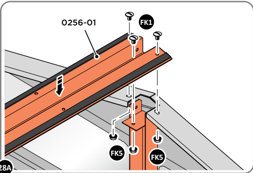
SLOT ROOF CHANNEL ASSEMBLY 0256-01 INTO ROOF SUPPORT. FIXING POINT (x3 EACH SIDE) USING FASTENERS DETAILED ABOVE.
