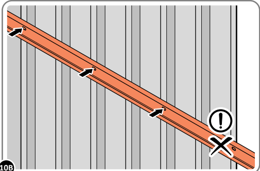
10B LOOSELY ATTACH AT x5 LOCATIONS INDICATED ONLY. IMPORTANT: DO NOT SECURE AT OUTER FIXING POINT INDICATED.
