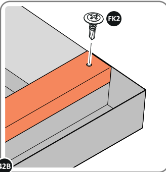
42B SECURE REAR ROOF CAP AT x8 LOCATIONS.
