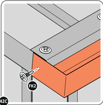
42C SECURE SLIDE ROOF GUTTER 0215-19 AT x2 LOCATIONS.
