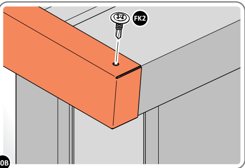
40B SECURE ROOF CAP AT x8 LOCATIONS INDICATED USING TYPICAL FIXING METHOD. PLEASE NOTE: THE FIXING USED IS A SELF DRILLING COMPONENT.
