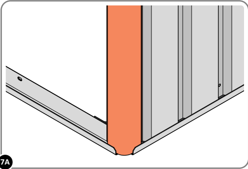
7A LOCATE CORNER POST 0205-14 AS SHOWN ABOVE.
