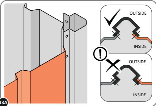
13A LOCATE FIRST WALL PANEL 0205-13 (1850 x 425mm) AS SHOWN ABOVE. IMPORTANT: ENSURE PANEL IS IN THE CORRECT ORIENTATION.
