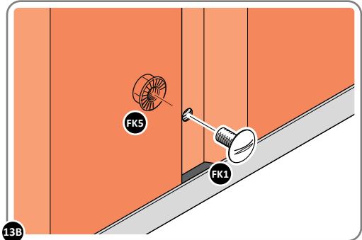
13B LOOSELY ATTACH WALL PANEL AT x2 LOCATIONS INDICATED ONLY. IMPORTANT: DO NOT SECURE ANY FIXING POINTS OTHER THAN THOSE INDICATED.
