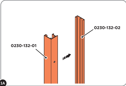
1A LOCATE AND SEPARATE BOTH LEG EXTRUSIONS AS SHOWN ABOVE.
