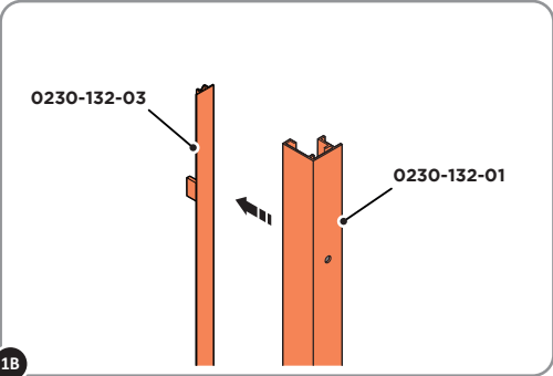
1B SEPARATE PLASTIC EXTRUSION FROM LEG EXTRUSION AS SHOWN ABOVE.
