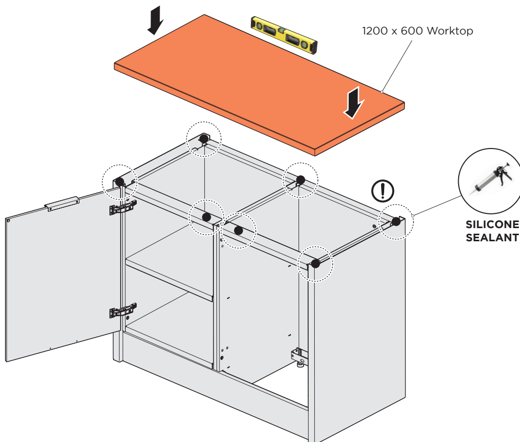
TYPICAL DOUBLE 1200 X 600 UNIT
