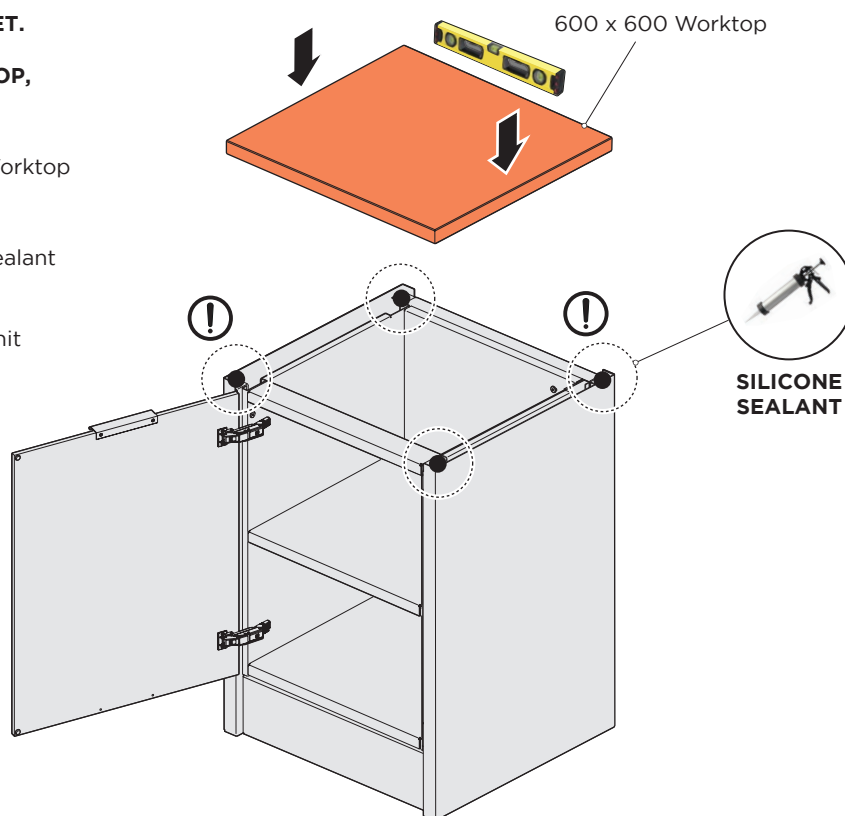
TYPICAL SINGLE 600 X 600 UNIT
