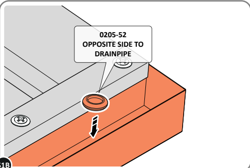
51B LOCATE CLOSED GROMMET INTO THE ROOF GUTTER ON THE OPPOSITE SIDE TO THE LOCATED DRAIN HOLE AS SHOWN ABOVE.
