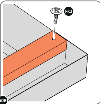
50B SECURE REAR ROOF CAP AT x10 LOCATIONS.
