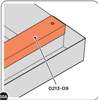
50A LOCATE REAR ROOF CAP 0213-09 ONTO REAR OF ROOF AS SHOWN ABOVE.
