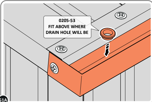
51A LOCATE AN OPEN GROMMET INTO THE ROOF GUTTER ABOVE WHERE THE DRAIN HOLE WILL BE LOCATED.
