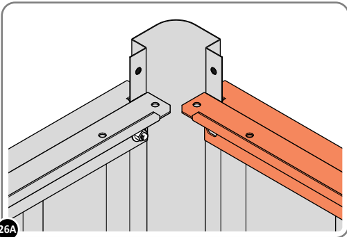
26A LOCATE LONG ROOF RAIL 0213-02 AS SHOWN ABOVE.
