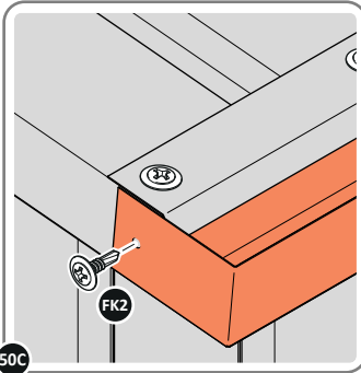
50C SECURE SLIDE ROOF GUTTER 0215-05 AT x2 LOCATIONS. PLEASE NOTE: THE FIXING USED IS A SELF DRILLING COMPONENT.
