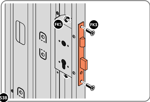
53B SECURE EURO MORTICE LOCK 0203-32 AT x2 LOCATIONS INDICATED ABOVE. SEE FOLLOWING DATA SHEET FOR COMPLETION OF MORTICE LOCK INSTALLATION.
