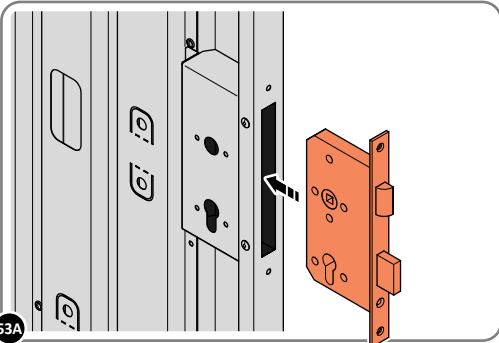
53A LOCATE EURO MORTICE LOCK 0203-32 RIGHT-HAND DOOR APERTURE AS SHOWN.
