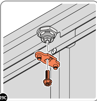
SECURE 2 POINT CAM 0206-28 ONTO T-HANDLE USING BOLT AS SHOWN FROM T-HANDLE ASSEMBLY.
