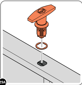
LOCATE T-HANDLE AND T-HANDLE GASKET 0204-58 INTO LID 0204-17 APERTURE AS SHOWN.
