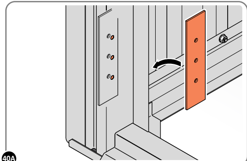
40A LOCATE DOOR HINGE PLATE 0203-37 WITHIN DOOR AS SHOWN.
