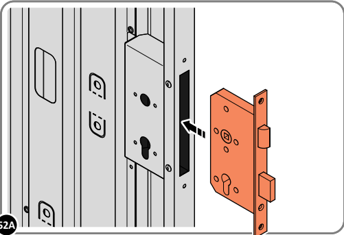
52A LOCATE EURO MORTICE LOCK 0203-32 RIGHT-HAND DOOR APERTURE AS SHOWN.
