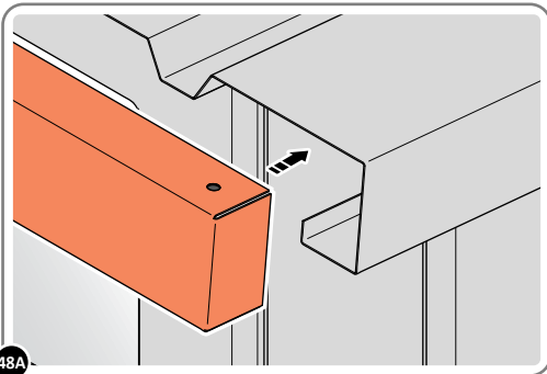
48A LOCATE ROOF CAP 0213-05 ONTO FRONT OF ROOF.
