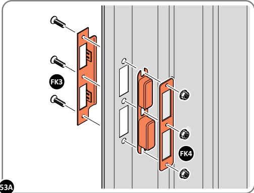
53A LOCATE AND SECURE EURO MORTICE LOCK 0203-32 AND CATCH PLATE COVER 0203-41 AS SHOWN ABOVE.
