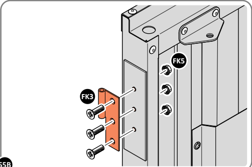
55B SECURE DOOR HINGE PLATE AND HINGE 0203-27 AND 0203-28 AS SHOWN. IMPORTANT: ENSURE CORRECT DOOR HINGE IS SECURED TO CORRECT DOOR.
