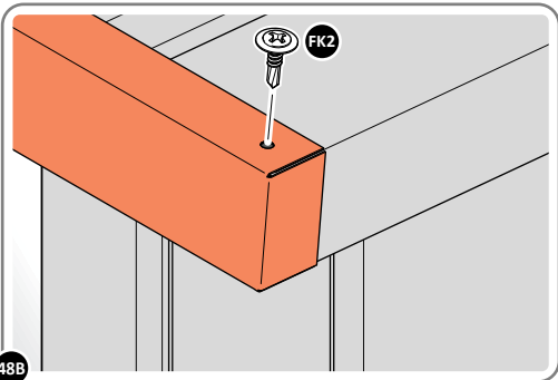
48B SECURE ROOF CAP AT x12 LOCATIONS INDICATED USING TYPICAL FIXING METHOD. PLEASE NOTE: THE FIXING USED IS A SELF DRILLING COMPONENT.
