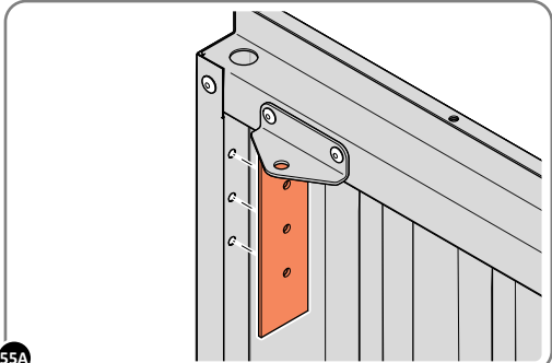
55A LOCATE DOOR HINGE PLATE 0203-37 WITHIN DOOR AS SHOWN.
