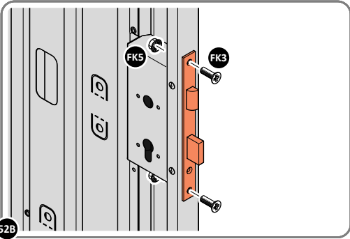
52B SECURE EURO MORTICE LOCK 0203-32 AT x2 LOCATIONS INDICATED ABOVE. SEE FOLLOWING DATA SHEET FOR COMPLETION OF MORTICE LOCK INSTALLATION.
