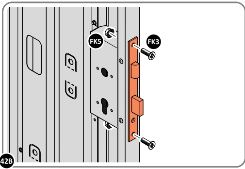
42B SECURE EURO MORTICE LOCK 0203-32 AT x2 LOCATIONS INDICATED ABOVE. SEE FOLLOWING DATA SHEET FOR COMPLETION OF MORTICE LOCK INSTALLATION.
